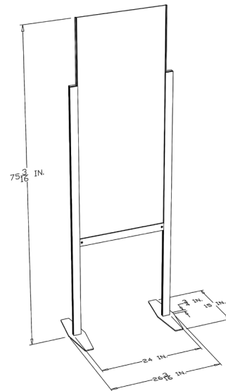
FLOOR STANDING SEPARATOR
