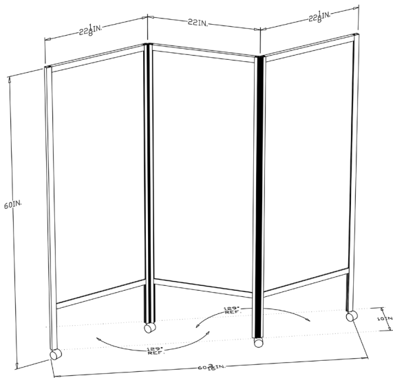
ACCORDION FOLDING DIVIDER FLUTED PLEXI WITH RAISED BOTTOM
